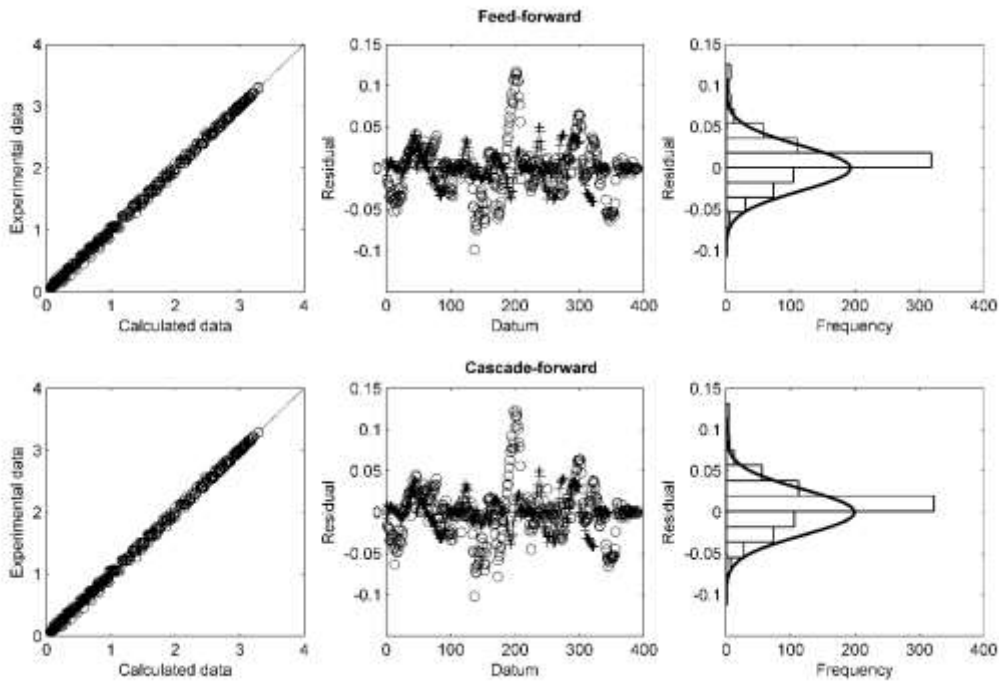
Figure 5. Residual analysis between the experimental and calculated drying curves for shrimp shell ( \circ ) and exoskeleton crab ( + ) using the best ANN architectures.
