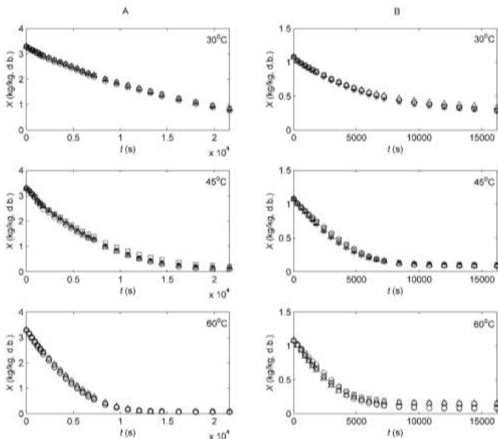
Figure 1. Drying kinetics curves for shrimp shell (A) and crab exoskeleton (B) at the different temperature levels. (○) sample 1, (Δ) sample 2, (□) sample 3 and (*) sample 4.
