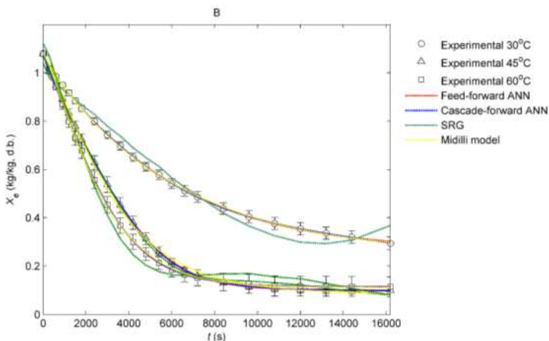
Figure 6. Comparison between the ANNs, SRG and thin-layer methods on the modelling of the drying rates of the shrimp shell (A) and crab exoskeleton (B).
