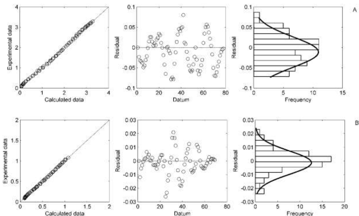
Figure 2. Residual analysis between the experimental and calculated drying curves using the best fitting models of Page for shrimp shell (A) and Midilli for crab exoskeleton (B).
