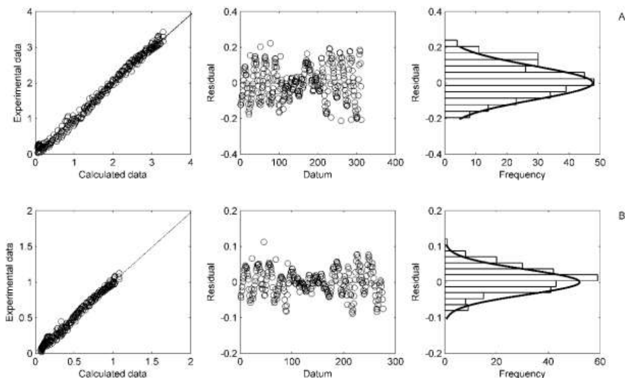
Figure 3. Residual analysis between the experimental and calculated drying curves for shrimp shell (A) and crab exoskeleton (B) using the stepwise fit regression models.
