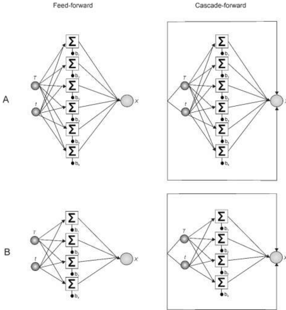
Figure 4. Architectures of the best ANNs for the simulations of the drying kinetics of shrimp shell (A) and crab exoskeleton (B).
